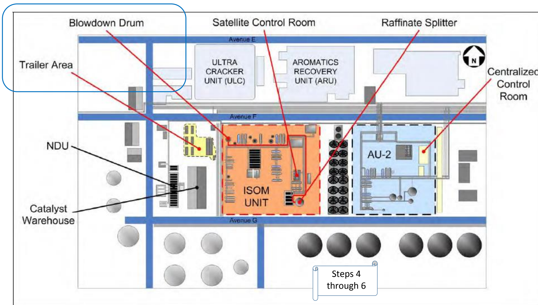
Figure 3 - ISOM Unit Site Layout for RAST BP Texas Case Study (From CSB Report)
