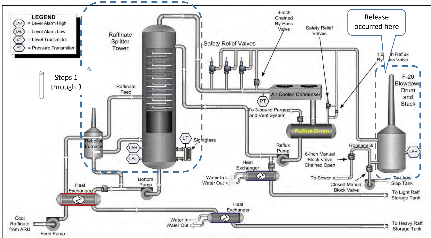
Figure 2 - Raffinate Splitter Tower System of the ISOM Unit (From CSB Report) for RAST BP Texas Case Study
