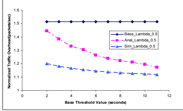
Figure 2. Normalized traffic overhead due to SeNDORComm and GenericComm (Base).
