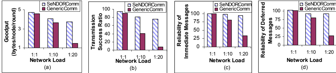
Figure 5. Behavior of SeNDORComm and GenericComm under varying load conditions on a 100 node network simulation.
