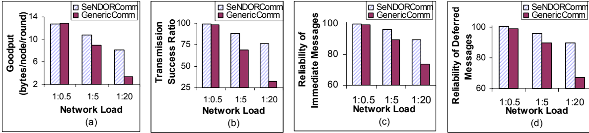
Figure 4. Behavior of SeNDORComm and GenericComm under varying load conditions on a 21 node test bed network
