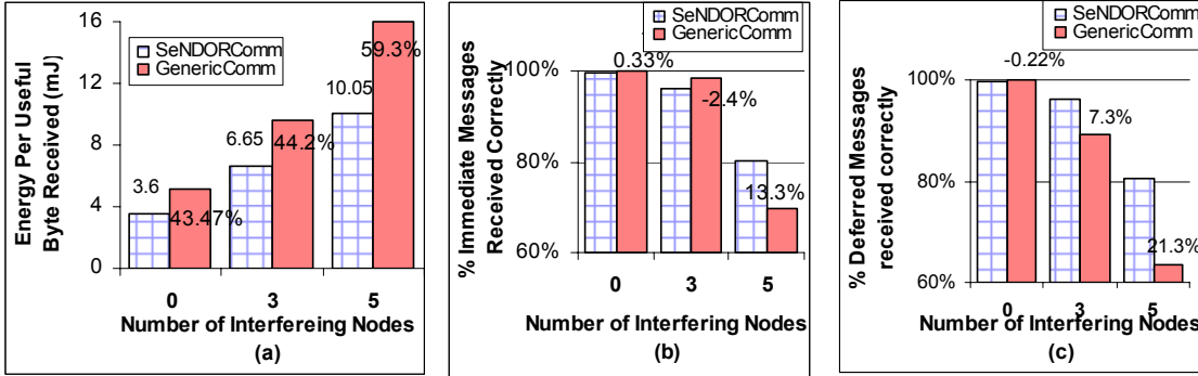
Figure 3. (a) Energy spent by the sender node per useful byte received for different levels of interference in network. (b) and (c) Fraction of immediate and deferred messages received successfully. The percentage numbers on GenericComm denotes the increase relative to the corresponding SeNDORComm case and in (a), the number on SeNDORComm denotes the absolute energy value.
