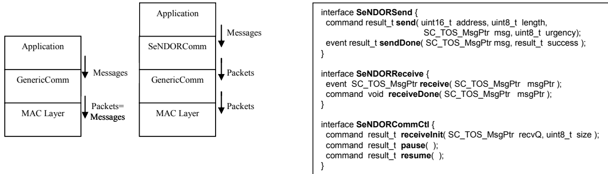
Figure 1. WSN application’s radio stack interface respectively without and with SeNDORComm (left). SeNDORComm Interfaces: Send, Receive, Control (right).
