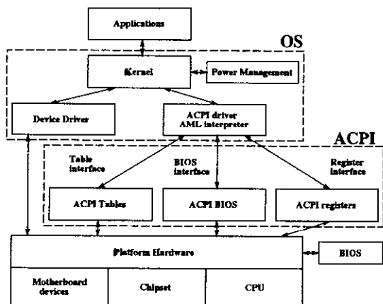
Figure 1: ACPI Interface and PC Platform
