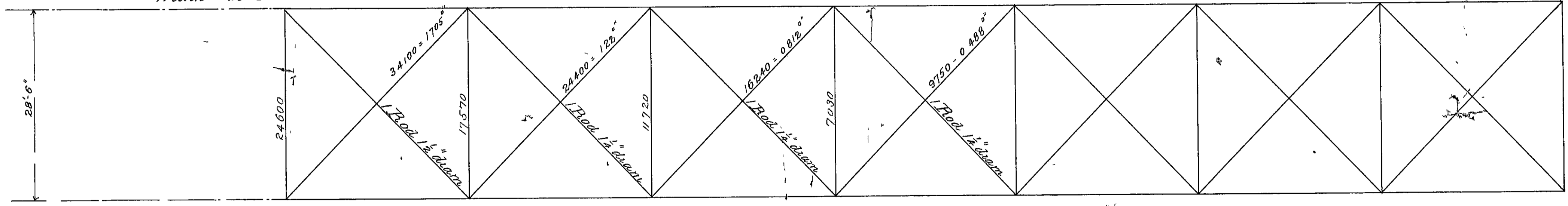
Top Lateral Bracing
