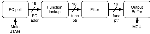
Figure 6. FPGA pipeline in PC polling mode.
