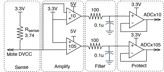
Figure 2. Simplified schematic of the energy monitoring circuit of the TDB.
