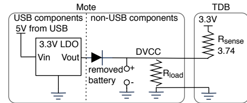
Figure 3. Simplified schematic of powering the mote through the TDB. The mote's battery should not be connected.
