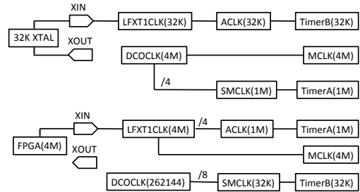
Figure 7. TinyOS clock module setup (top) and modified setup for PC polling (below).
