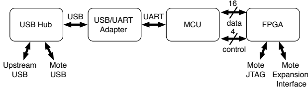
Figure 5. Hardware architecture of the TDB.
