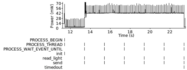
Figure 12. Watchpoint trace of application level functions and threads of a sender node in the Contiki tracking application.
