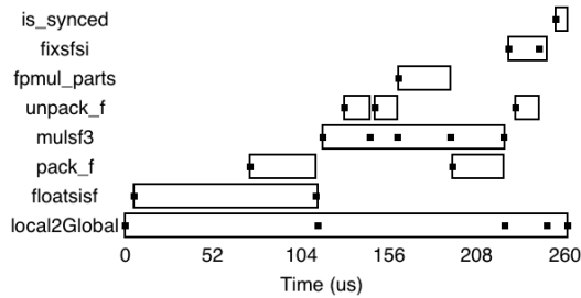
Figure 14. Trace of the functions invoked in one execution of the local2Global function. Filled squares represent data collected from PC polling, and open rectangles represent the inferred executions of each function.
