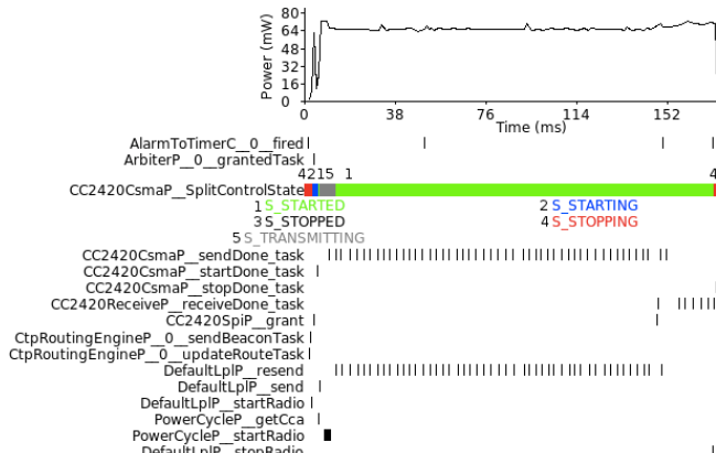
Figure 10. Watchpoint trace of task executions with the startRadio bug fixed.
