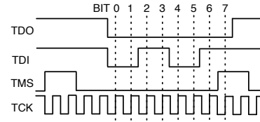
Figure 4. Timing example for shift IR. The byte 0xCC is shifted in on TDI while 0x00 is shifted out on TDO.
