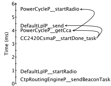
Figure 11. Execution timeline that causes task spinning.
