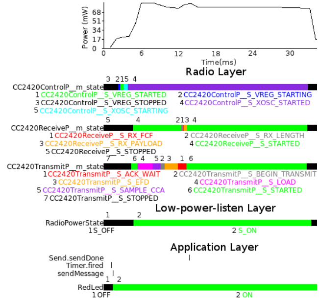
Figure 8. Watchpoint trace of states when sending a message in TestNetworkLpl, showing the application, low-power-listening, and radio layers. The number above each state’s timeline corresponds to the numbering of the states under the timeline. For example, in the low-power listen layer, state 1 is S_OFF and 2 is S_ON; at the beginning the state is 1, then an extended period of state 2, followed by a return to state 1.
