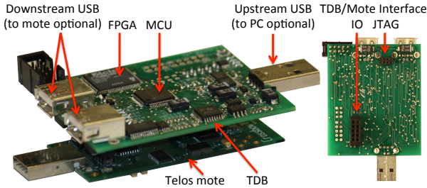
Figure 1. The Telos Debug Board (TDB) with a Telos Rev B mote underneath, and the underside of the TDB (right).
