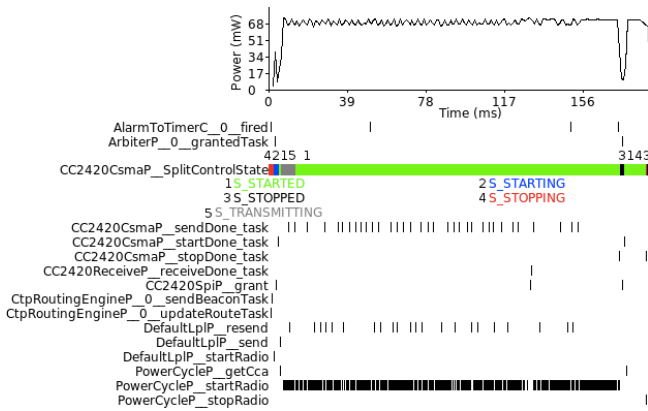
Figure 9. Watchpoint trace of task executions during a radio start event. The PowerCycleP_startRadio task is called over 3000 times due to a bug in the handling of the CC2420CsmAP_SplitControlState.
