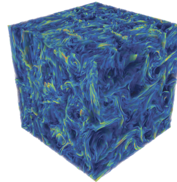
How do turbulent plasmas behave in star formation?
