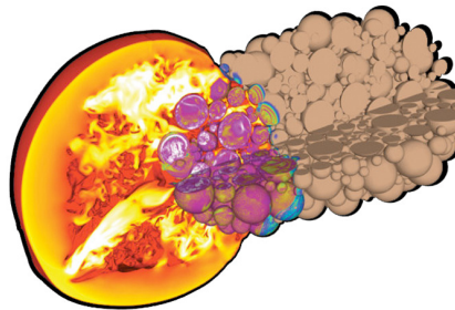
How would the detonation of a nuclear energy source affect an incoming asteroid?
