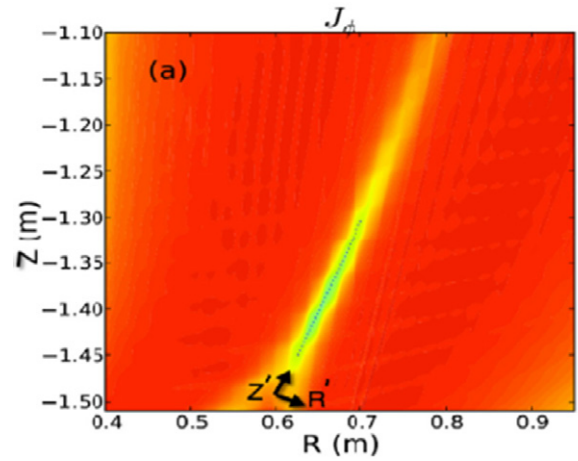
Figure 4. Toroidal current in the reconnection region. [14, 15]. (Copyright 2013, American Institute of Physics.)
