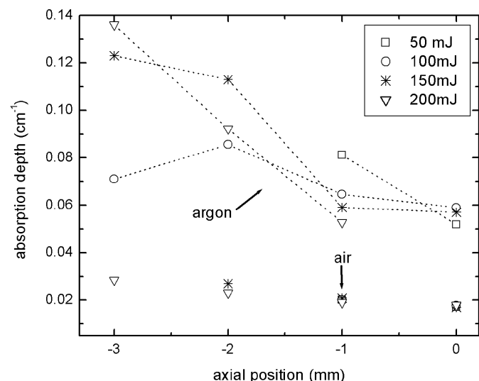
FIG. 7. The estimated inverse bremsstrahlung absorption depth for argon and air sparks for different laser energies. The data points without lines represent the air spark while data points with dashed curves represent the argon spark.
