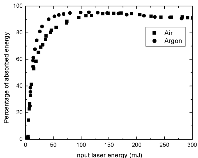
FIG. 9. The percentage of absorbed and scattered laser energy by the air and argon sparks obtained from Fig. 8 plotted against incident laser energy.
