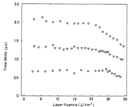
Fig. 3. Variation of time delays with laser fluence for the second peak at distances ( \square ) 5 mm, ( \nabla ) 10 mm and ( \circ ) 15 mm (helium pressure 0.5 Torr).
