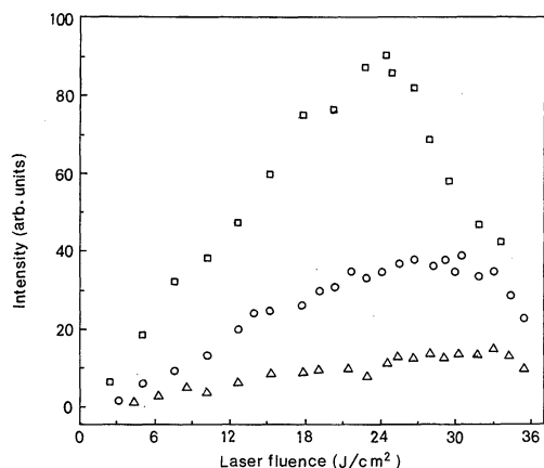
Fig. 5. Change in intensity for second peak with respect to laser fluence at different distances ( \square ) 5 mm, ( \circ ) 10 mm and ( \triangle ) 15 mm (pressure 0.5 Torr).
