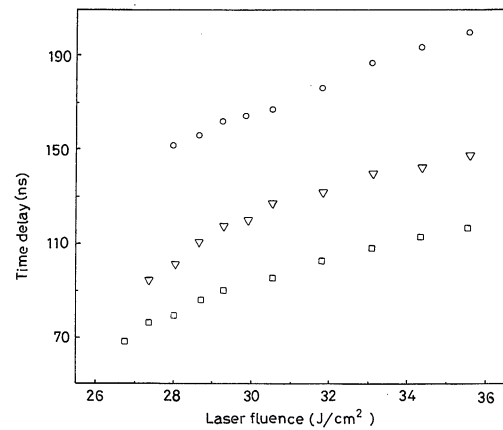
Fig. 2. Variation of time delays with laser fluence for the first peak at distances ( \square ) 5 mm, ( \nabla ) 10 mm and ( \circ ) 15 mm (helium pressure 0.5 Torr).
