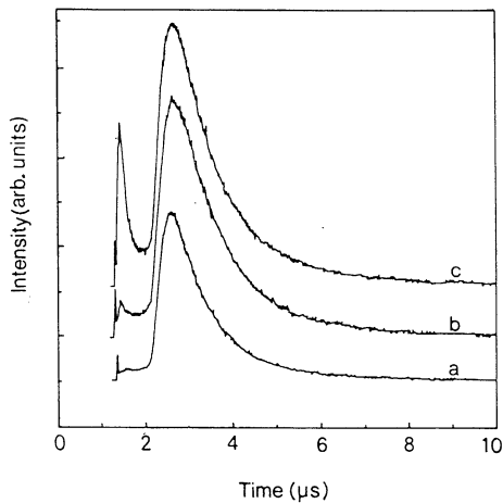
Fig. 1. Intensity variation of spectral emission with time for C_2 observed at 1 cm away from the target for laser fluences (a) 26.7 J/cm^2 (b) 27.4 J/cm^2 and (c) 28 J/cm^2 (helium pressure 0.5 Torr).
