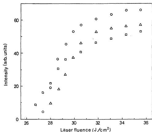
Fig. 4. Change in intensity for first peak with respect to laser fluence at different distances ( \square ) 5 mm, ( \circ ) 10 mm and ( \triangle ) 15 mm (pressure 0.5 Torr).
