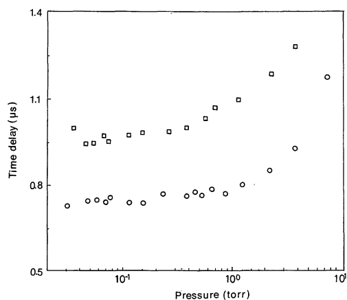
Fig. 7. Dependence of time delays of second peak on ambient helium pressure (○) 5 mm and (□) 8 mm (laser fluence 30 \text{ J/cm}^2 ).
