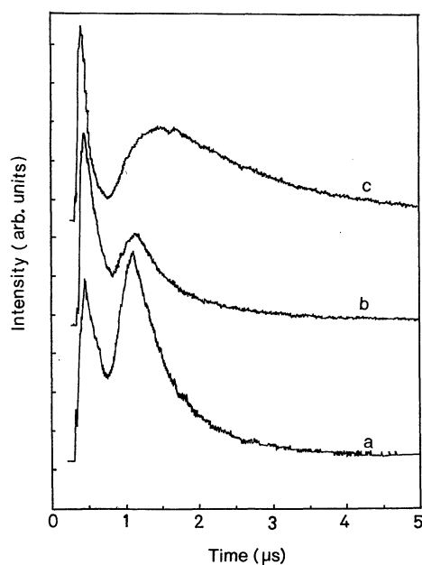
Fig. 8. Intensity variation of spectral emission with time for \text{C}_2 observed at 8 mm away from the target at different ambient helium pressures (laser fluence 30 \text{ J/cm}^2 ) (a) 0.05 Torr, (b) 0.8 Torr and (c) 7.5 Torr.
