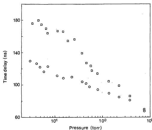
Fig. 6. Dependence of time delays of first peak on ambient helium pressure (○) 5 mm and (□) 8 mm (laser fluence 30 \text{ J/cm}^2 ).
