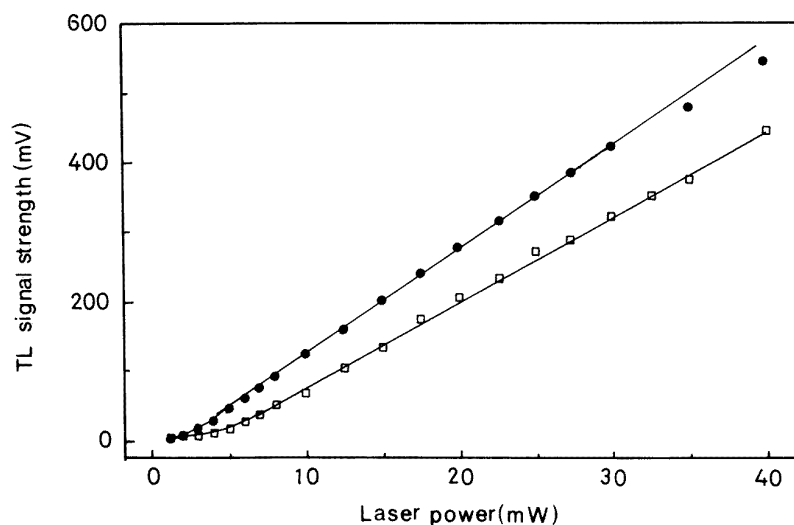
Figure 3. The variation in thermal signal strength with laser power for concentrations (○) 8.6 \times 10^{-4} and (□) 8.6 \times 10^{-6} \text{ mol l}^{-1} .
