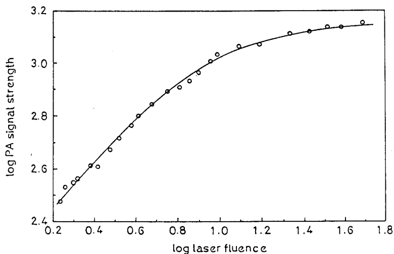
Fig. 2. Log-log plot of PA signal strength with laser filter.
