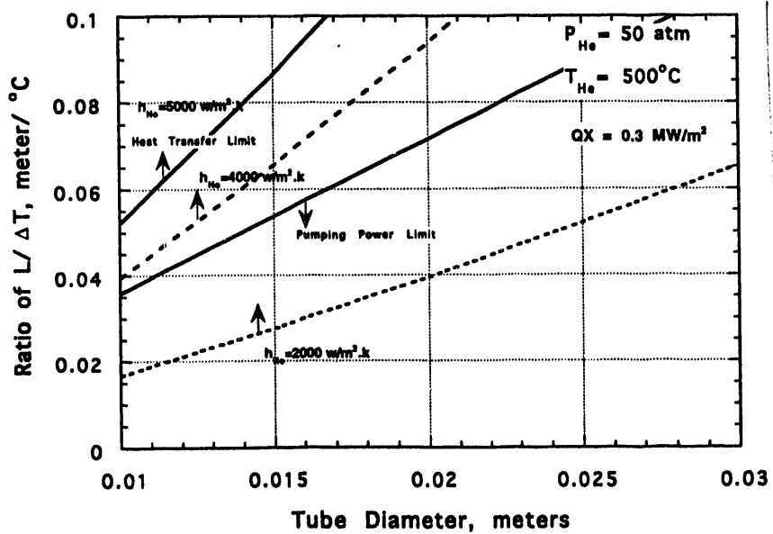
Fig. 2 Design limitations for helium pressure of 5 MPa.
