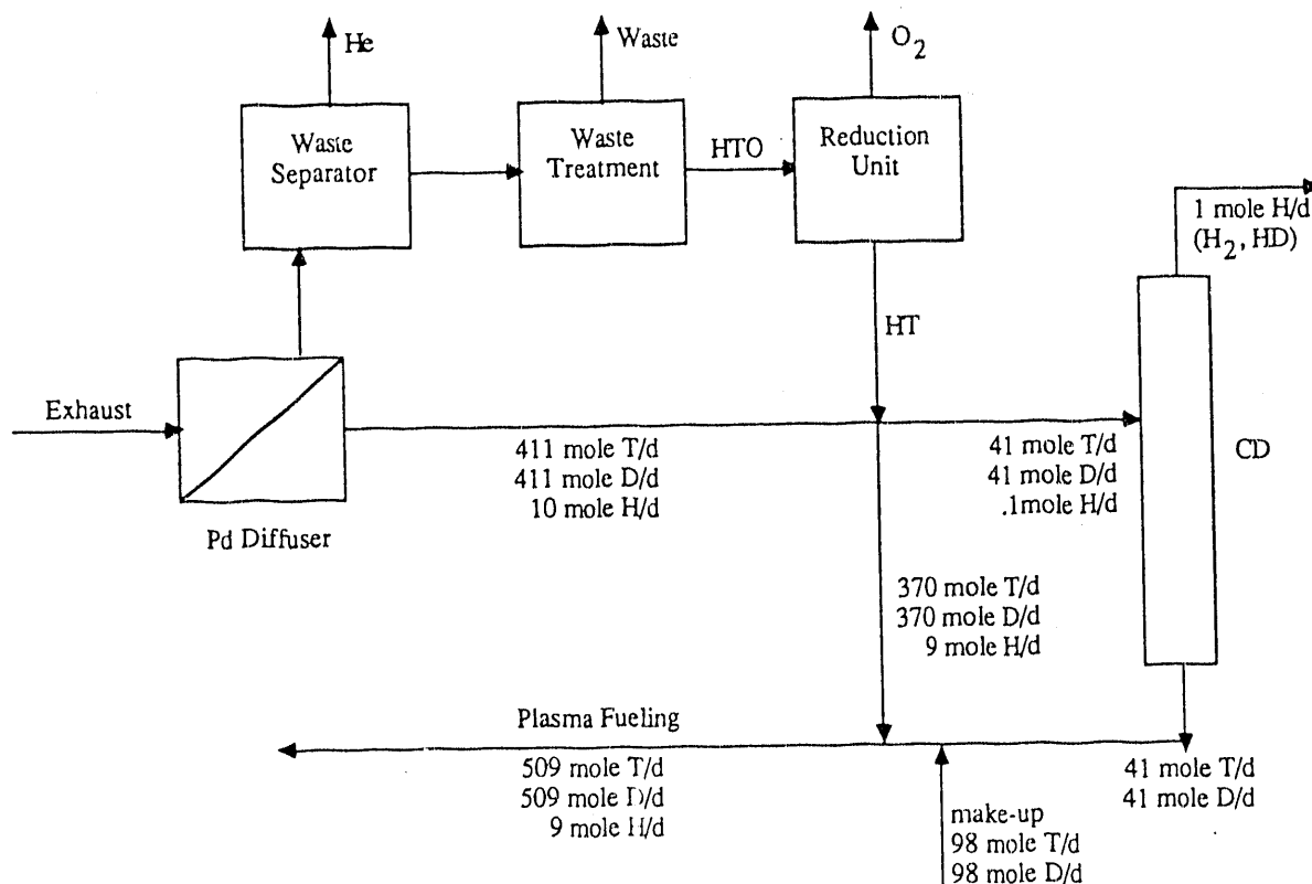
Figure 2. ARIES-I fuel processing flow diagram.
