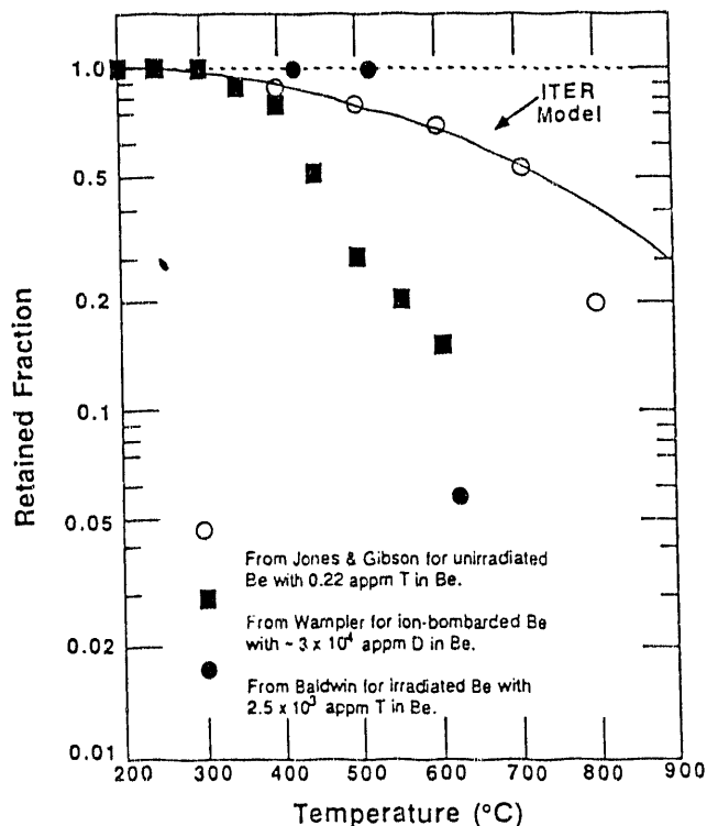
Fig. 1 Fraction of "trapped" hydrogen isotope in Be as a function of annealing temperature for 25-100 hour anneals of unirradiated Be soaked with tritium and 10 minute anneals of deuterium-ion-implanted Be.
