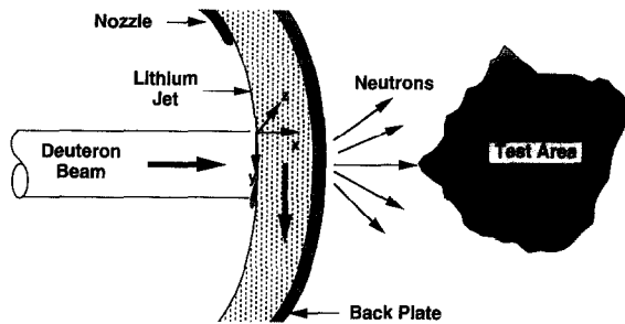
Fig. 1. Schematic illustration of beam on target interaction assembly in a neutron-source test facility.
