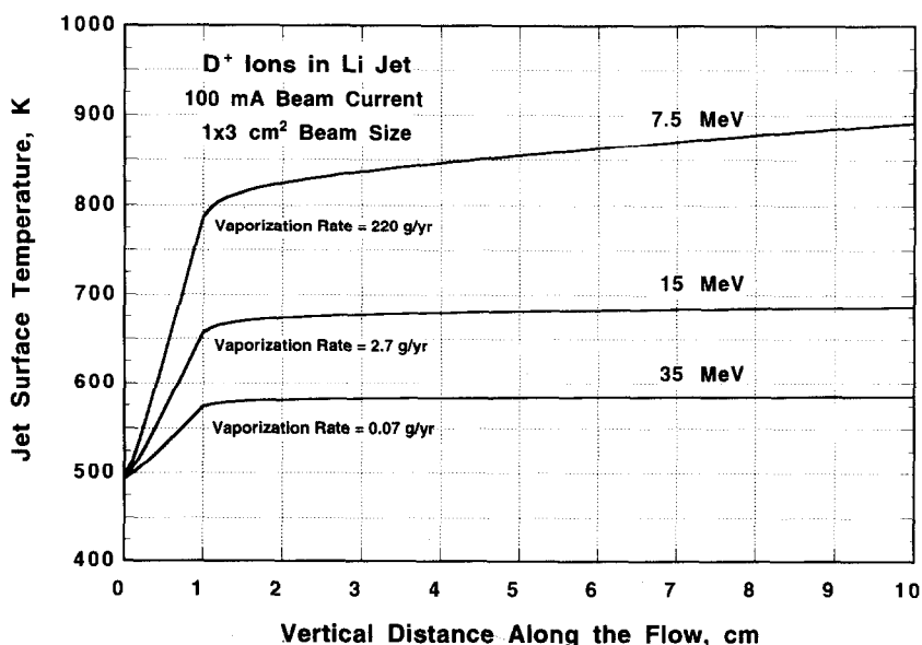
Fig. 6. Jet surface temperature and vaporization rate at different beam energies.
