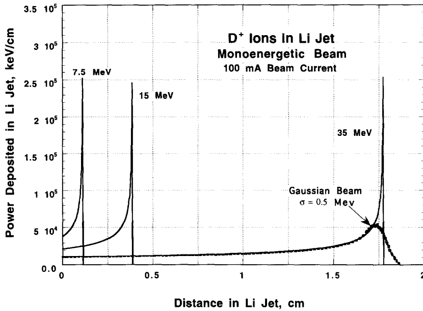
Fig. 2. Energy-loss profile of deuteron beam in Li target.
