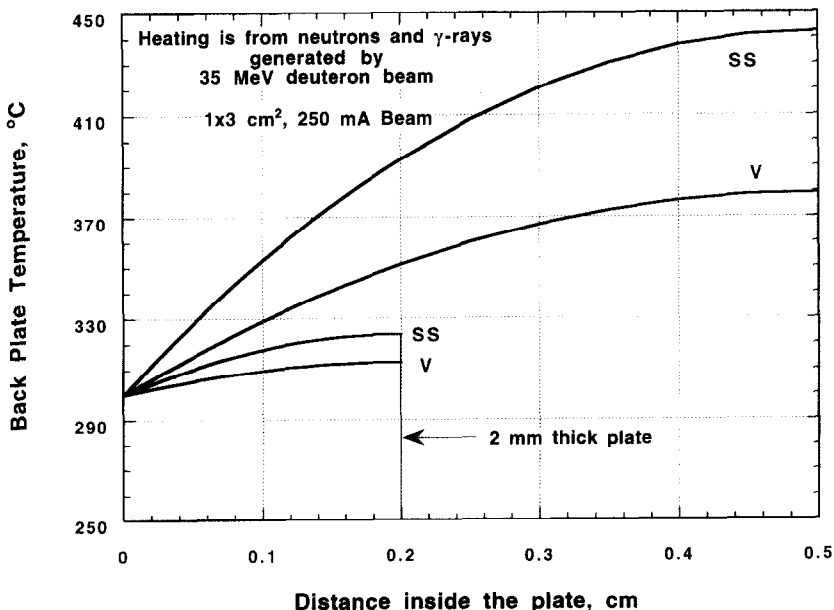
Fig. 8. Back-plate temperature distribution for stainless steel (SS) and vanadium (V) plates at different plate thicknesses.
