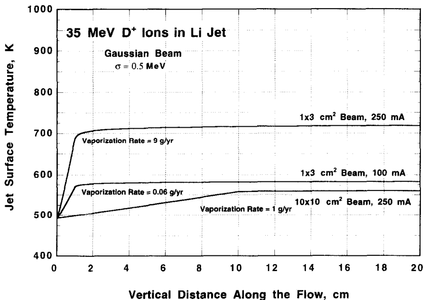
Fig. 5. Jet surface temperature and vaporization rate at different beam sizes and currents.
