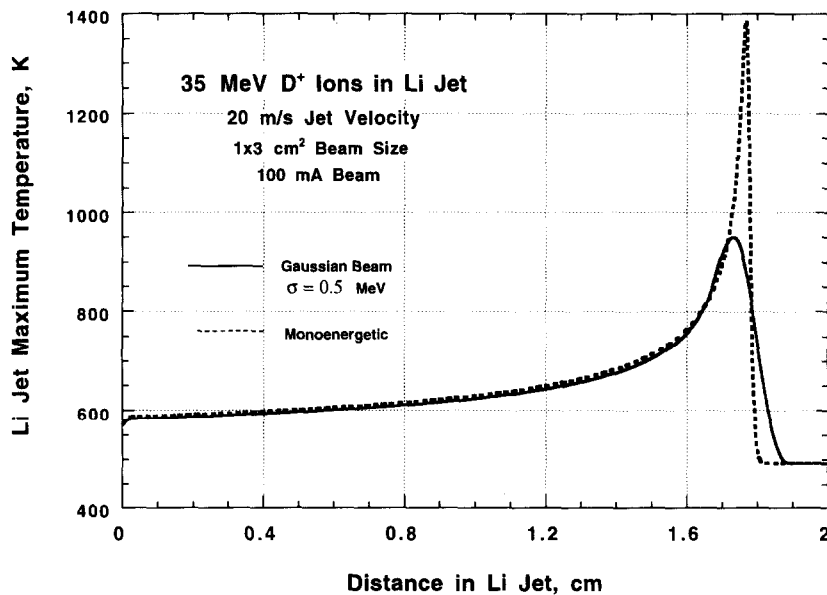
Fig. 3. Spatial distribution of Li maximum temperature for Gaussian and monoenergetic beam profiles.
