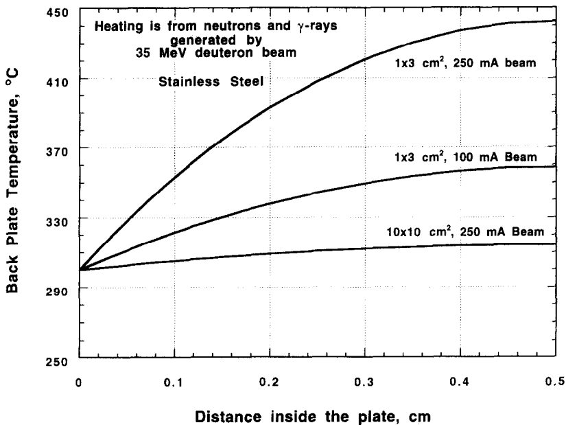
Fig. 7. Spatial distribution of stainless steel back-plate temperature at different beam parameters.
