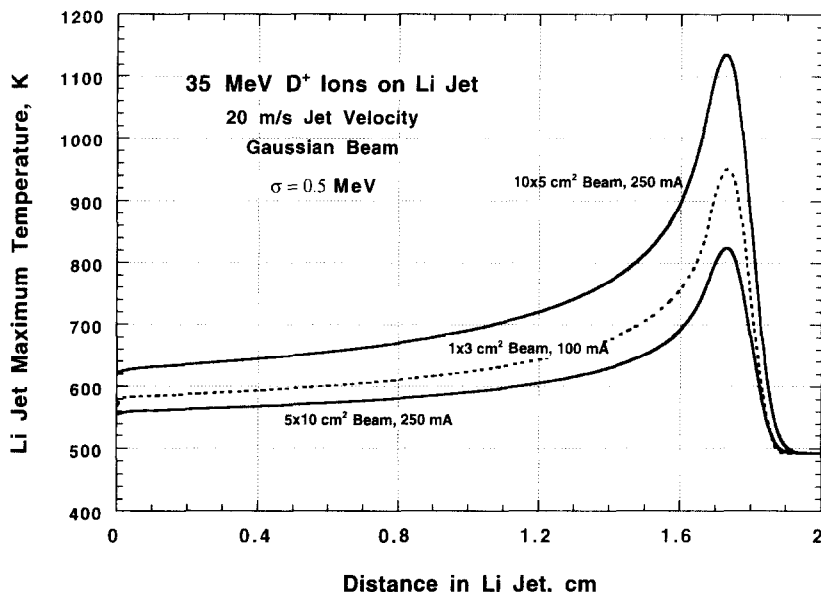
Fig. 4. Spatial distribution of Li maximum temperature for different beam sizes and currents.
