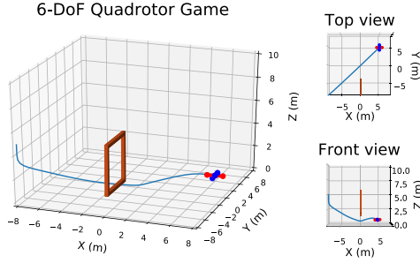
Fig. 12. Six-DoF quadrotor game. A human participant teaches the quadrotor to learn a cost function by applying directional corrections through a keyboard (see the instruction in Table II). The goal is that the quadrotor can fly from the initial position (in the bottom left), go through a gate (colored in brown), and land on the target (in the upper right). Note that we have no knowledge about the gate.
