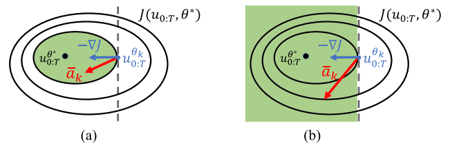
Fig. 3. Magnitude corrections vs. directional corrections. Contours (circles) and desired trajectory \mathbf{u}_{0:T}^{\theta^*} (black dot) of the true cost function J(\theta^*) are plotted. (a) Allowable region of magnitude corrections; green region (a sub-level set) indicates all allowable magnitude corrections \bar{\mathbf{a}}_k that satisfy J(\mathbf{u}_{0:T}^{\theta_k} + \bar{\mathbf{a}}_k, \theta^*) < J(\mathbf{u}_{0:T}^{\theta_k}, \theta^*) . (b) Allowable region of directional corrections; green region (half of the input space) indicates all allowable directional corrections \bar{\mathbf{a}}_k that satisfy \langle -\nabla J(\mathbf{u}_{0:T}^{\theta_k}, \theta^*), \bar{\mathbf{a}}_k \rangle > 0 .
