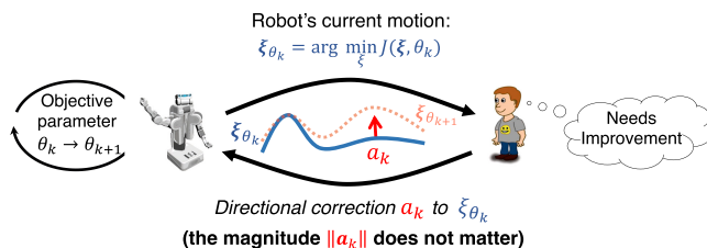
Fig. 1. Illustration of learning from directional corrections proposed in this article. The robot’s current motion \xi_{\theta_k} optimizes an objective function parameterized by \theta_k . A human user applies a directional correction a_k to \xi_{\theta_k} . Note that the magnitude \|a_k\| of this correction does not matter. After receiving a_k , the robot updates its objective function parameter to \theta_{k+1} . This motion correction update process repeats until the convergence of the objective function parameter.
