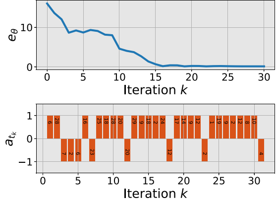
Fig. 7. Learning from simulated directional corrections for the pendulum. The upper panel shows the weight error e_\theta = \|\theta - \theta^*\|^2 versus iteration. The bottom shows the simulated directional correction \mathbf{a}_{t_k} (positive or negative sign) at each iteration k ; here, the value in each bar is t_k , which is randomly drawn from a uniform distribution over horizon [0, 30] .
