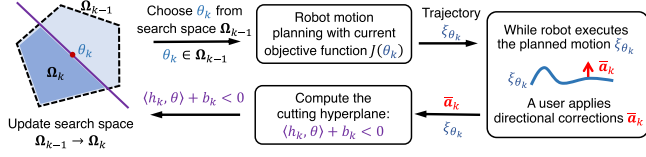
Fig. 2. Overview of the proposed algorithm.
