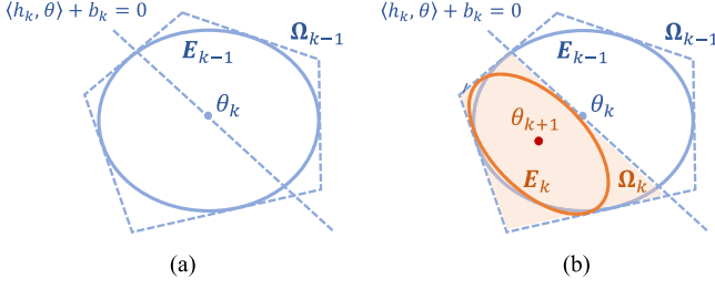
Fig. 6. Illustration of choosing \theta_{k+1} as the center of MVE E_k inscribed in the weight search space \Omega_k . (a) Center of MVE in \Omega_{k-1} . (b) Center of MVE in \Omega_k .
