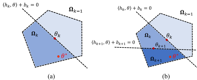
Fig. 4. Illustration of updating \Omega_k . (a) At k th iteration. (b) At (k+1) th iteration.
