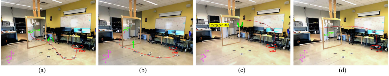
Fig. 17. Results of a real-world quadrotor learning from human directional corrections. Here, the quadrotor trajectory is marked in red lines. The initial position (red circle) and target position (green circle) are also marked. (a) Iteration k = 1 . (b) Iteration k = 2 . (c) Iteration k = 3 . (d) Iteration k = 4 . In (a), during the quadrotor flying, the human user applied a torque correction in the opposite of the x -axis, shown by the green arrow. In (b), during the quadrotor flying, the human user applied an upward thrust correction (in green arrow) in z -axis. In (c), the quadrotor detected a potential collision with the left pillar of the gate and thus triggered an emergence stop. But before the emergence stop, the human user had already applied a positive x -axis (in green arrow) torque to correct the quadrotor. In (d), the quadrotor successfully learned a cost function to fly from the initial position, go through the gate, and finally reach the target position.
