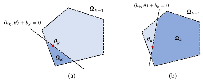
Fig. 5. Illustration of how different human directional corrections \bar{\mathbf{a}}_k affect the cut of the weight search space \Omega_{k-1} . (a) Large cut from \Omega_{k-1} . (b) Small cut from \Omega_{k-1} .
