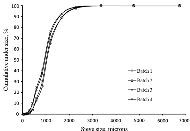
Fig. 2. Particle size distribution of DDGS products.
