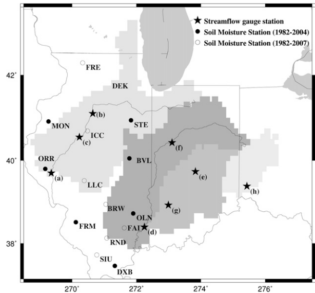
FIG. 1. Location of watersheds, streamflow gauging stations, and soil moisture observation sites used in model calibration and evaluation. Gauging stations in Illinois unless otherwise noted: (a) Illinois River at Valley City; (b) Illinois River at Henry; (c) Illinois River at Kingston Mines; (d) Wabash River at Mt. Carmel; (e) White River at Indianapolis, IN; (f) Wabash River at Lafayette, IN; (g) White River at Newberry, IN; and (h) Miami River at Hamilton, OH. Soil moisture sites include (1) BVL, (2) DXB, (3) BRW,* (4) ORR, (5) DEK, (6) MON, (8) ICC,* (9) LLC,* (10) FRM, (11) Carbondale* (SIU), (12) OLN, (13) FRE,* (14) RND,* (15) STE, and (34) Fairfield* (FAI). Model simulations for the drought analysis were limited to Indiana and Illinois. The asterisk indicates the soil moisture observations used were for 1982–2007; otherwise, observations used were for 1982–2004.
