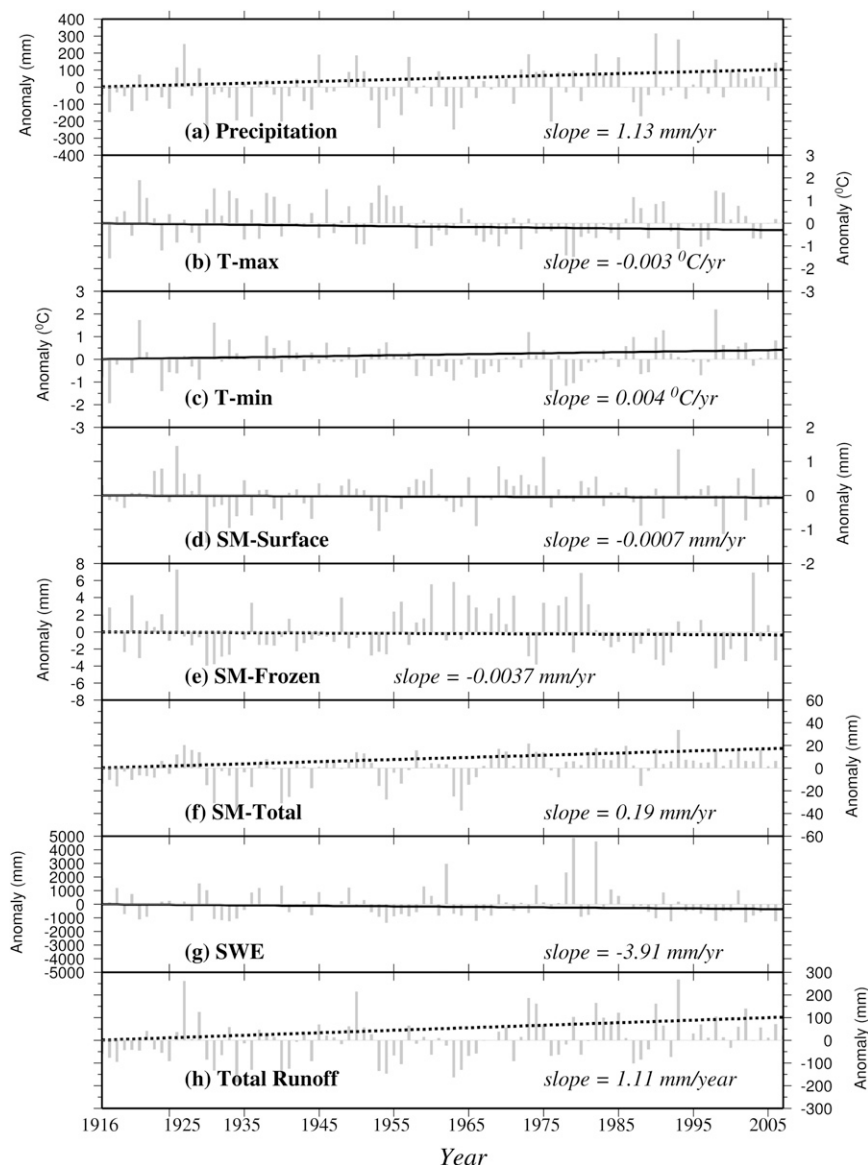
FIG. 7. Trend analysis using annual anomalies of domain-averaged (a) P , (b) T-max, (c) T-min, (d) SM-Surf, (e) SM-Frozen, (f) SM-Total, (g) SWE, and (h) total runoff. Dashed lines indicate statistically significant trends at a 5% significance level; solid lines indicate nonsignificant trends.
