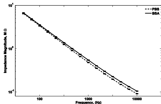
Fig. 2: Impedance magnitude spectrograms obtained from electrodes in PBS (dashed line) and BSA solution (solid line) in a log-log scale. The spectrograms demonstrate increased impedance magnitude in the BSA solution across the frequency spectrum.
