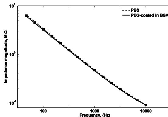
Fig. 3: Impedance magnitude spectrograms for electrodes in PBS (dashed line) and BSA solution after coating with PEG (solid line) in a log-log scale. The spectrograms show a slight decrease in the impedance magnitude in the BSA solution with the PEG coating at the lower frequencies. This decrease in impedance is not obvious at higher frequencies. The spectrograms indicate that the PEG coating has modulated the degree of protein adsorption onto the surface of the electrode sites.
