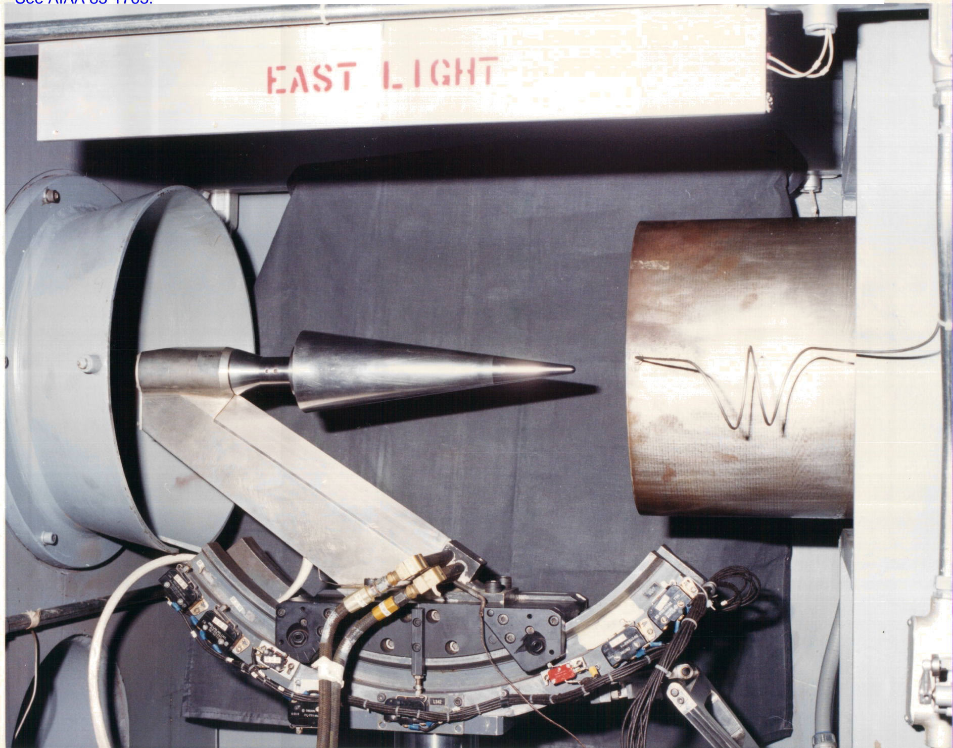
Stetson's Blunt Cone in High Reynolds Number Mach 6 Tunnel at Air Force Lab in Dayton, from Ken Stetson 5/2003. See AIAA 83-1763.
