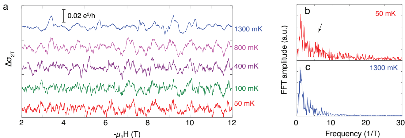
FIGURE 4 | UCF under different temperatures. (a) Field dependence of \Delta\sigma_{2T} for the 50 \mu\text{m} devices at different temperatures. (b,c) Fast Fourier transform of \Delta\sigma_{2T} at 50 and 1300 mK, respectively. The black arrow indicates the frequency corresponding to the high-frequency fluctuations.
