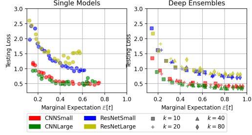
Figure 9: The illustration of the relation between the expected testing loss \mathbb{E}_{\mathcal{X}}[\mathcal{L}] and the marginal expectation \mathbb{E}_{\mathcal{X}}[t] , where models are from (a) single models with varying capacities (b) deep ensembles with varying member #. Each color represents a model family. In particular, in (b), different marker shapes indicate different k \in [10, 20, 40, 80] of the ensembles.
