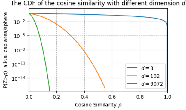
Figure 22: The relation between the probability \mathbb{P}(Z > \rho) and the cosine similarity value \rho .
