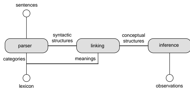
Figure 3: The cognitive architecture used by MAIMRA.
