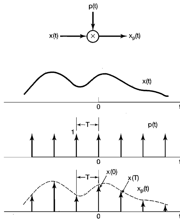
Figure 7.2 Impulse-train sampling.
