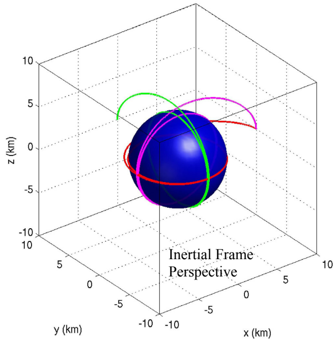
FIGURE 2 – OFL Controlled Response of Deputy Spacecraft Over 180 Days as Determined in the Ephemeris Model of the Sun-Earth/Moon System
