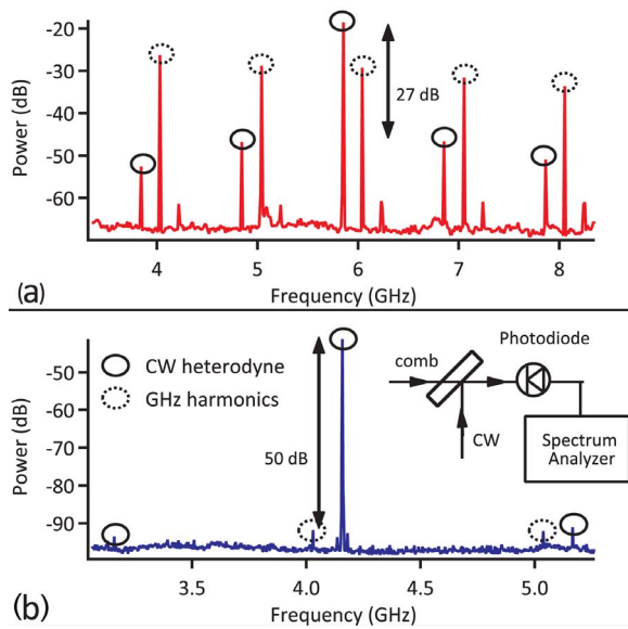
Fig. 4. (Color online) (a) Heterodyne beat with the single-pass cavity output. In addition to the beat notes indicated by solid circles, harmonics of the 1 GHz repetition rate are evident, as indicated by the dotted circles. The largest peak in the figure is the beat of the cw laser against a comb tooth aligned to the cavity resonance. The off-resonant comb teeth are suppressed by 27 dB. (b) cw heterodyne beat with the double-pass cavity output. The off-resonant mode suppression is 50 dB.
