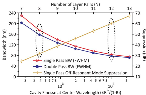
Fig. 2. (Color online) Simulation of quarter-wave stack mirrors and associated FP cavities. The coupling bandwidth (BW) decreases with increasing cavity finesse owing to the increased sensitivity to dispersion. Double-pass suppression is not shown, as it is exactly double the single-pass suppression, e.g., 60 dB versus 30 dB.
