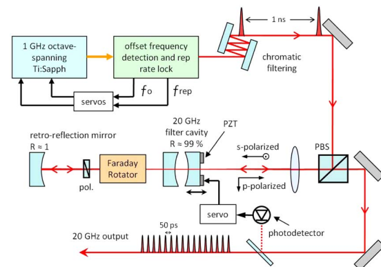
Fig. 1. (Color online) Stabilized 1 GHz input frequency comb is filtered by double passing through a 20 GHz FP cavity. The 20 GHz cavity is locked through the comb using a piezoelectric transducer behind one of the mirrors.
