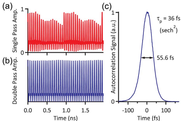
Fig. 5. (Color online) (a) Single-pass cavity time-domain signal with 30% amplitude modulation caused by the transmission of off-resonant comb modes. (b) Double-pass cavity time-domain signal showing less than 2% modulation. (c) Intensity autocorrelation trace showing a pulse width of 36 fs after compression by SF10 prisms. The transform limit is 30 fs.
