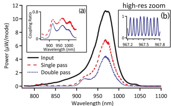
Fig. 3. (Color online) Input and output spectra for single- and double-pass cavities (power per mode). Most of the input bandwidth (50 nm FWHM) is coupled for both cases, giving output bandwidths of \sim 40 nm (FWHM). (a) Coupling ratio of output over input power per mode. Single pass shows 124 nm (FWHM) coupling bandwidth. Double pass shows 104 nm (FWHM) coupling bandwidth. (b) Zoomed view of high resolution (0.02 nm) optical spectrum analyzer trace showing individually resolved modes at 20 GHz.
