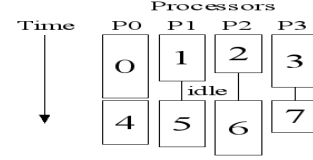
Figure 2: Load imbalance: Strict cyclic dispatch order inherent in the architecture leads to load imbalance.
