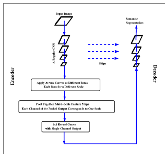
Figure: Fourth Generation Networks for Semantic Segmentation
